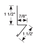
EAVE TRIM
