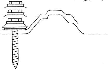
ROOFING - EAVE AND END LAPS
