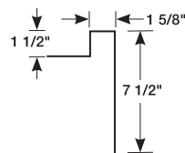
POST TRIM
